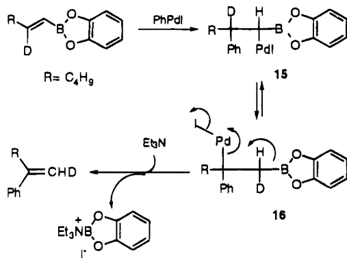
Figure 2. Addition–elimination mechanism for head-to-tail coupling.
