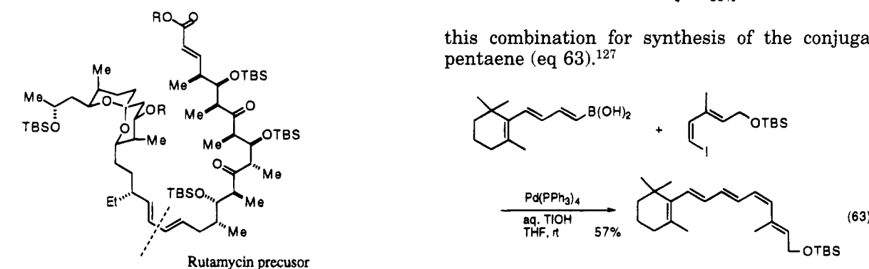
Figure 9. The coupling reactions induced by TIOH.
